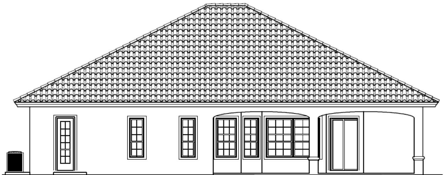
Rear Elevation
